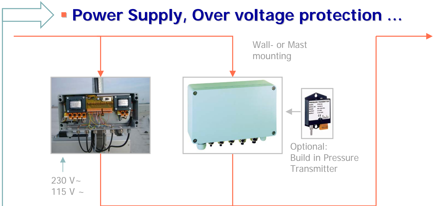
Connection Boxes with integrated Over voltage protection, Power Supply and Signal distribution.
